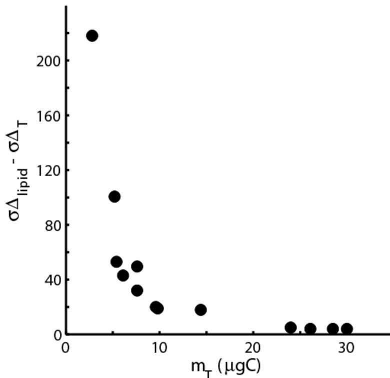
Figure 3 Difference between AMS facility-reported uncertainty ( \sigma_{\Delta_T} ) and total propagated uncertainty ( \sigma_{\Delta_{lipid}} ) plotted against total sample mass ( m_T ). The data include 3 unpublished measurements of bacterial fatty acids not included in Table 3.
