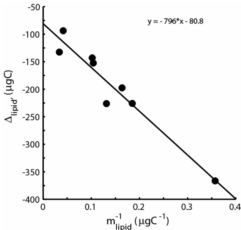
Figure 2 Plot of \Delta^{14}\text{C} measurements of lipid samples corrected for combustion blank and HPLC blank ( \Delta_{\text{lipid}} ) vs. 1/m_{\text{lipid}} ( m_{\text{lipid}} = m_T - m_{\text{CB}} - m_{\text{LC}} ). Equation of regression line corresponds to Equation 10. R^2 = 0.93 .
