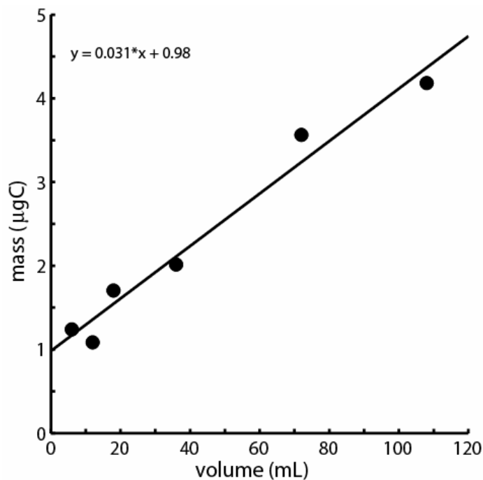
Figure 1 Plot of volume of mass vs. HPLC effluent volume for combusted HPLC effluent samples. Linear regression was used to determine the mass of combustion and HPLC blanks. R^2 for linear regression: 0.97.
